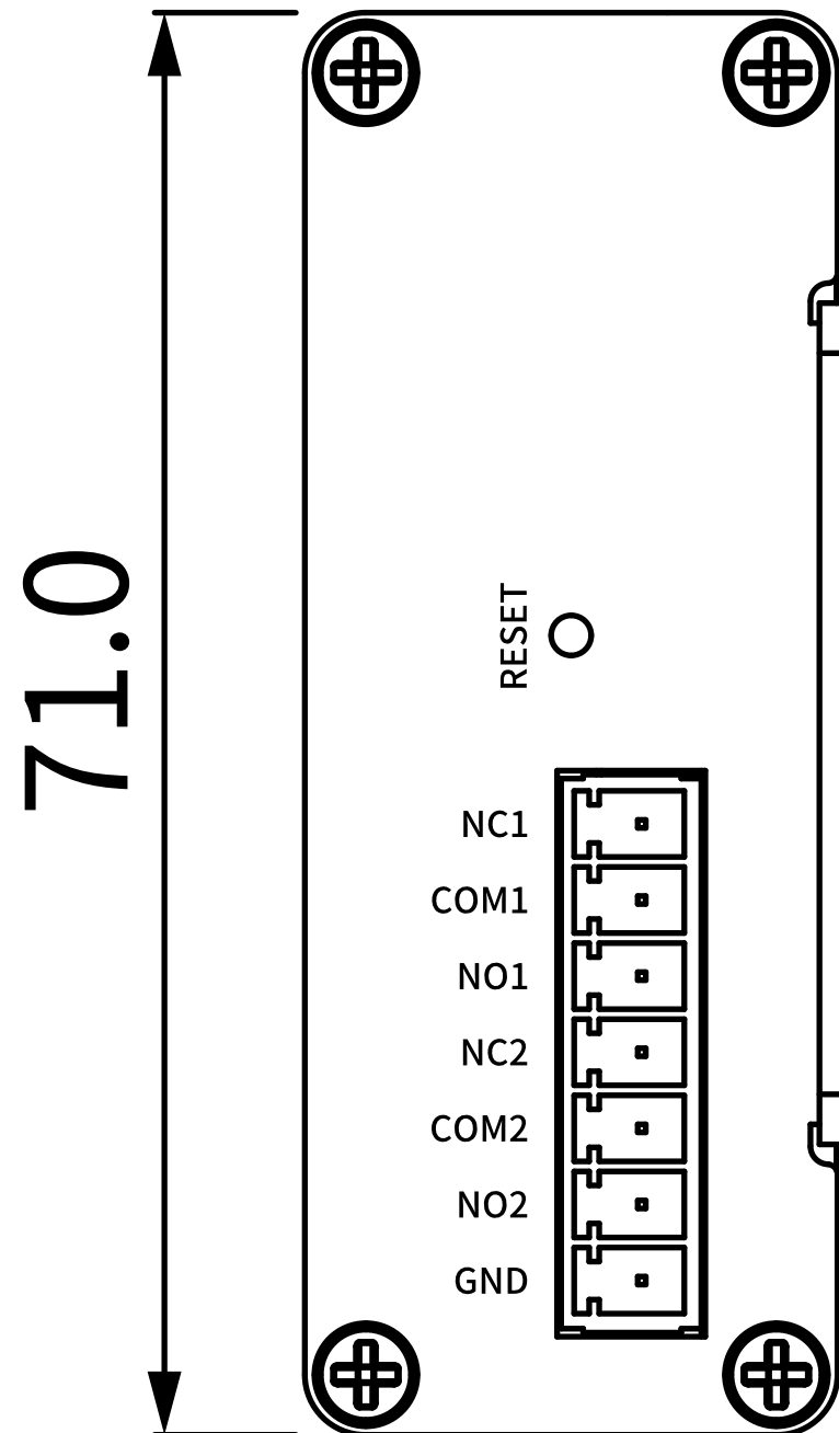
2 RIGHT VIEW
