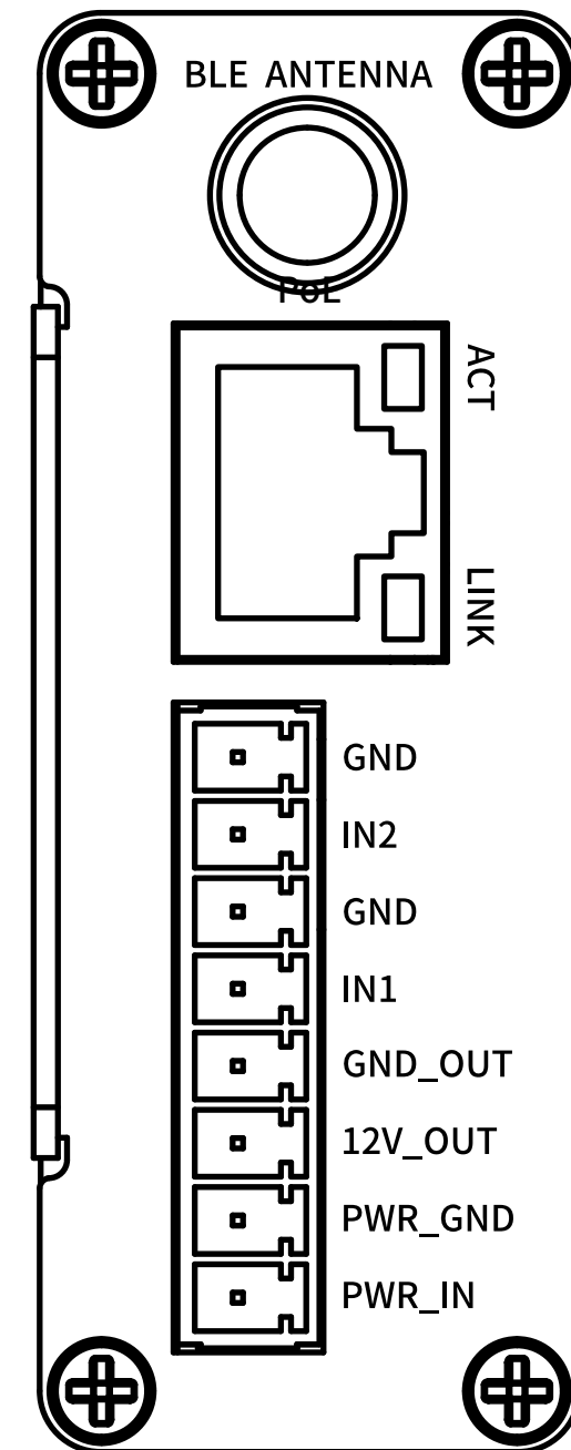
3 LEFT VIEW
