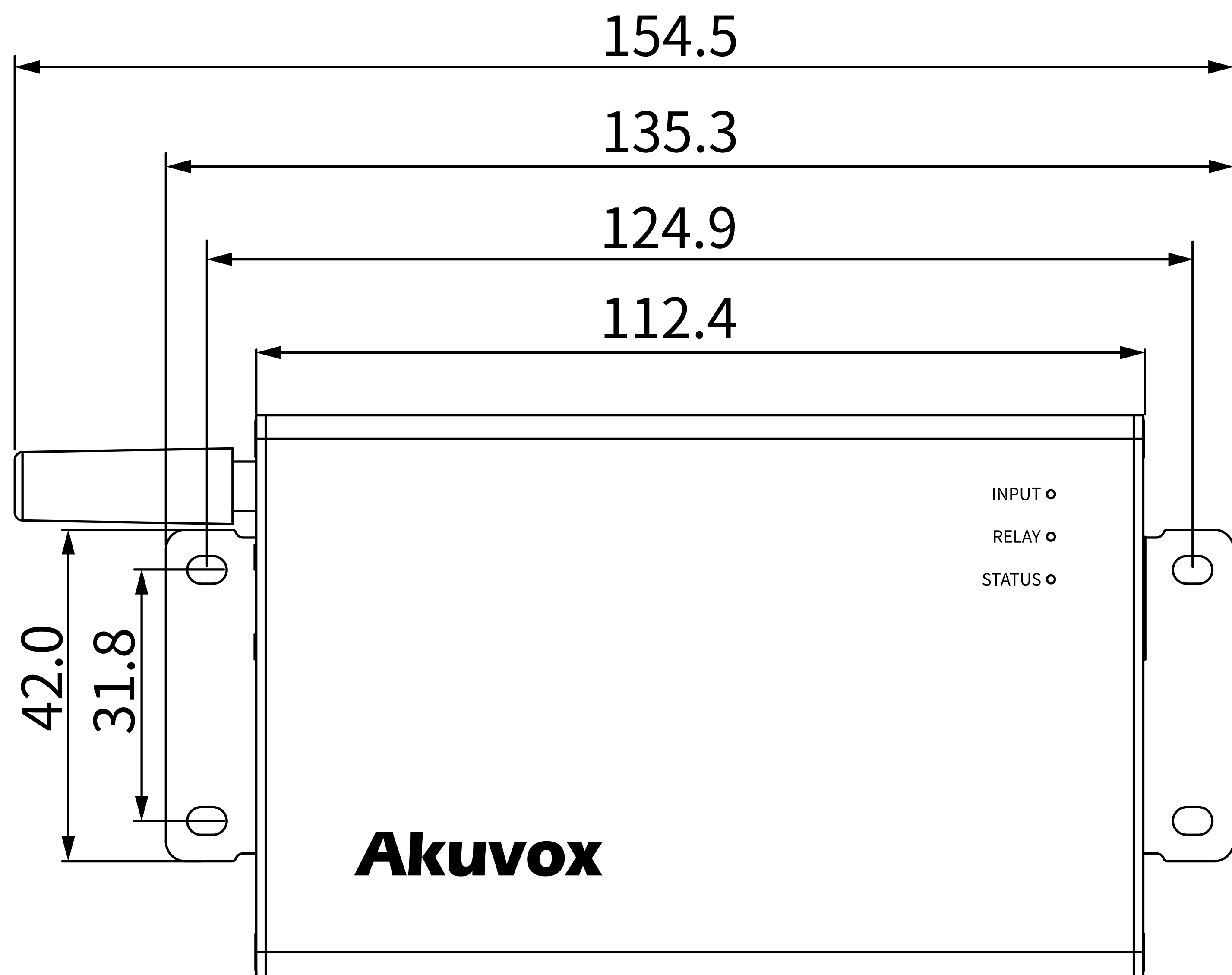
1 FRONT VIEW
