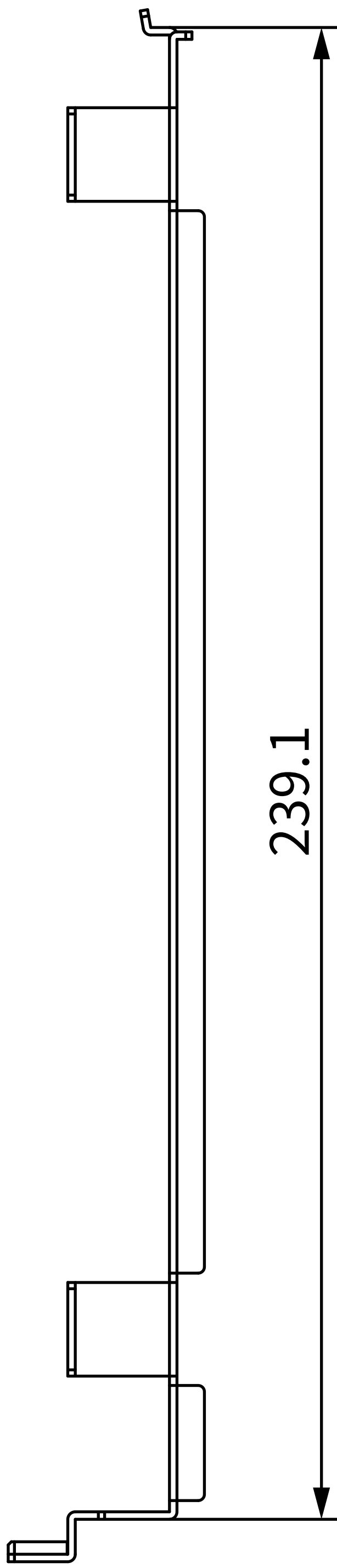
2 RIGHT VIEW
