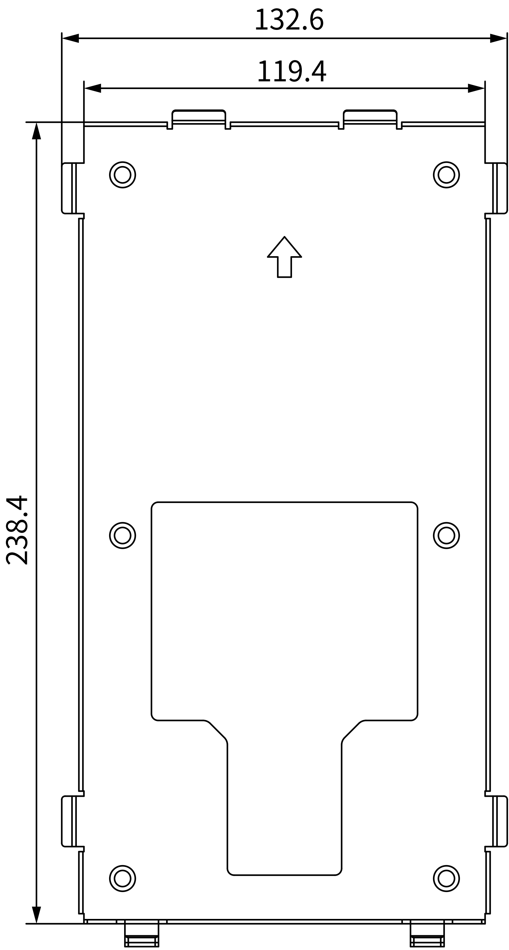
1 FRONT VIEW
