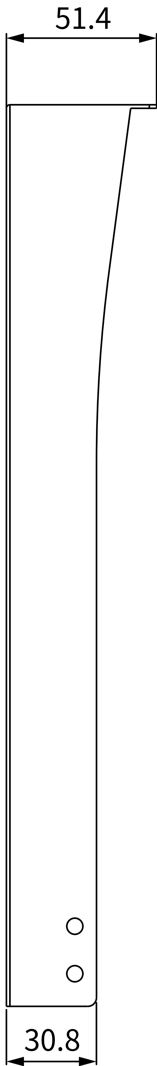
3 LEFT VIEW
