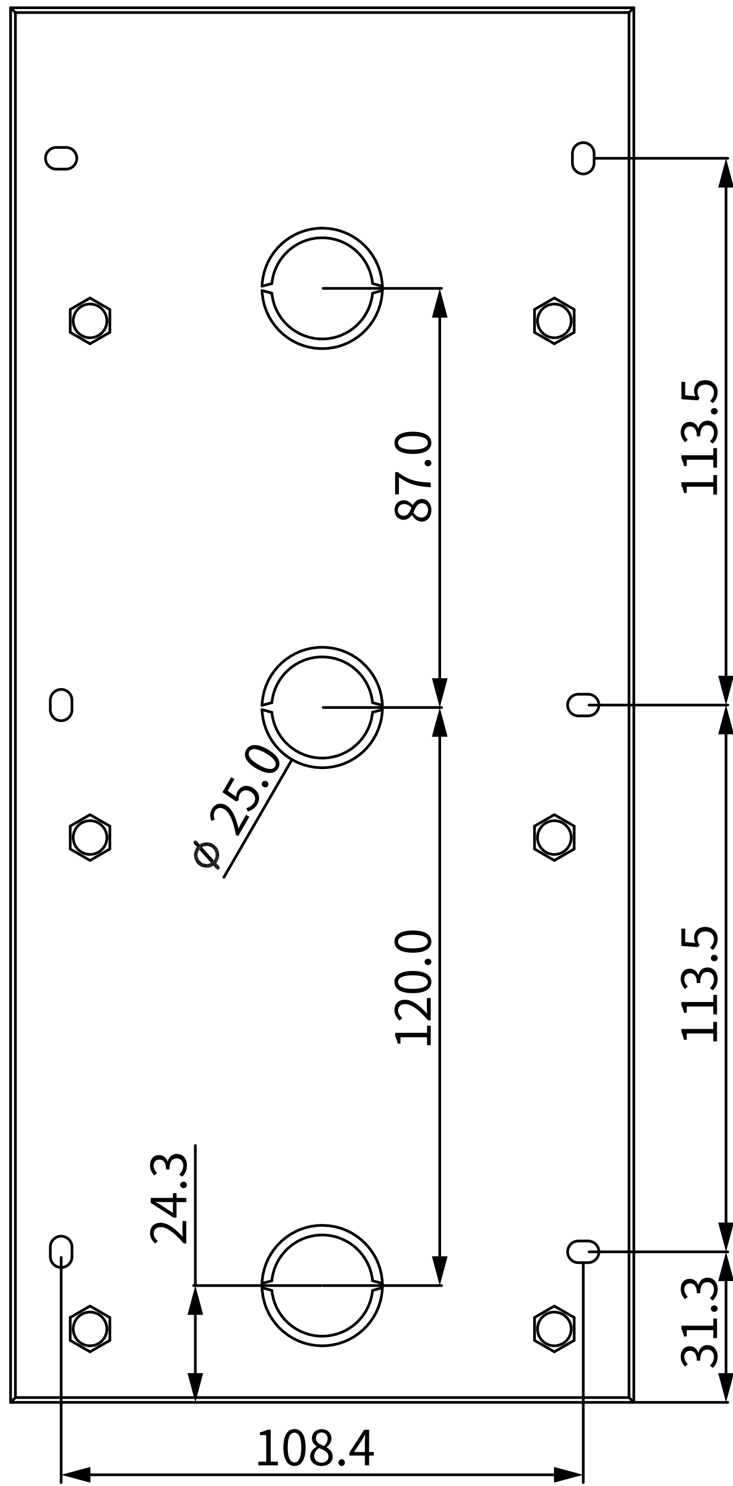
4 BACK VIEW
