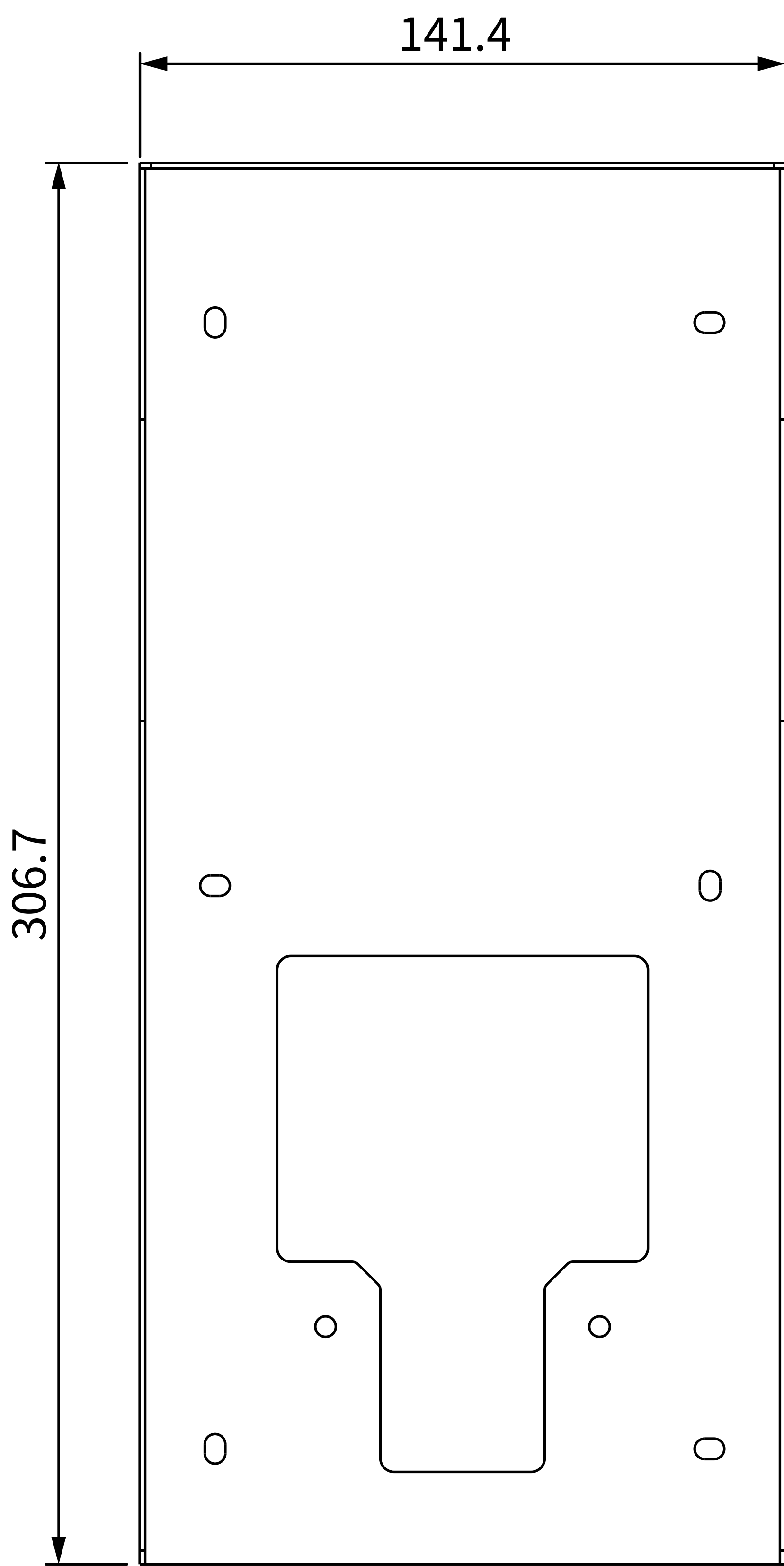
1 FRONT VIEW
