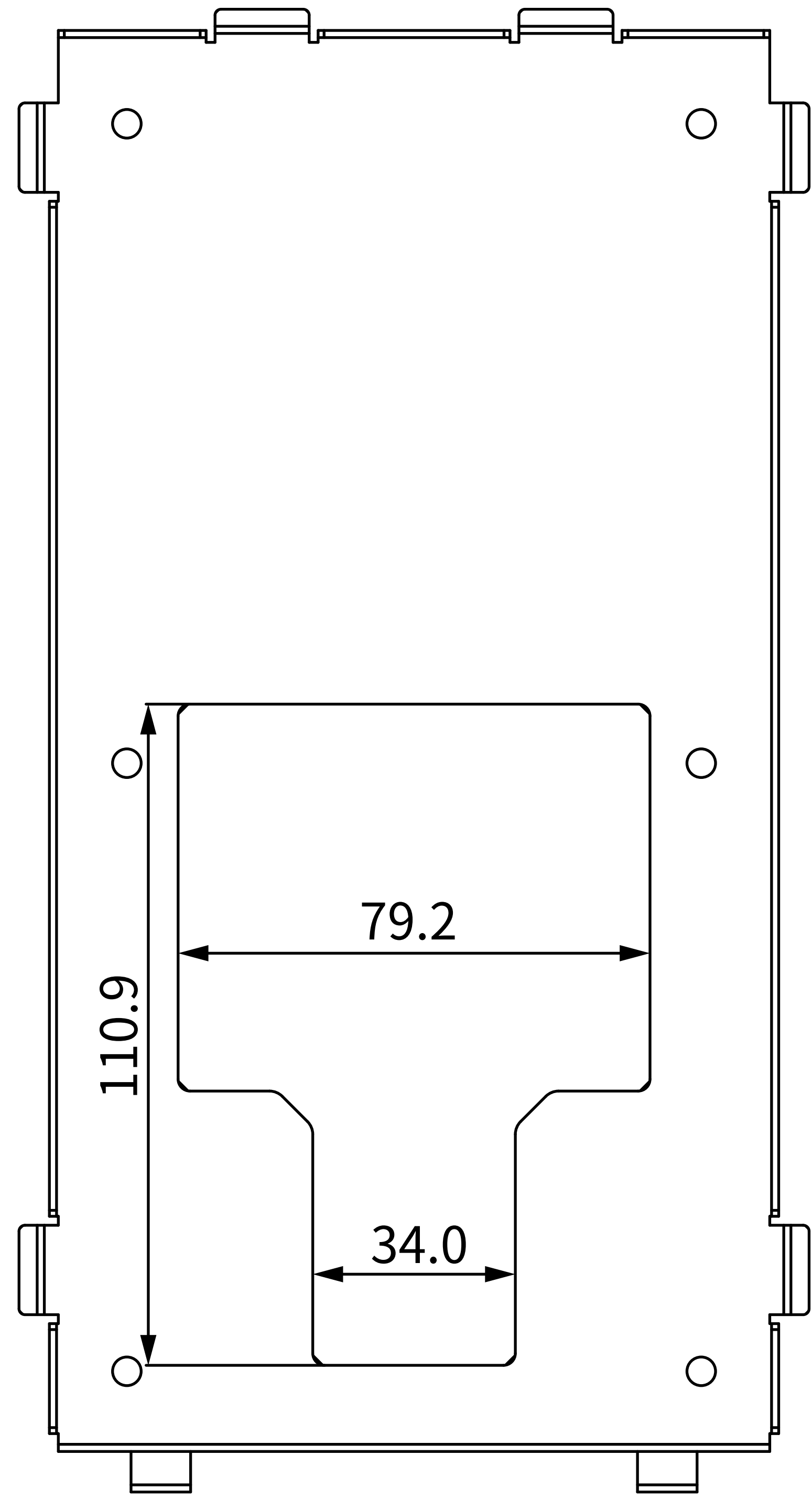
4 BACK VIEW
