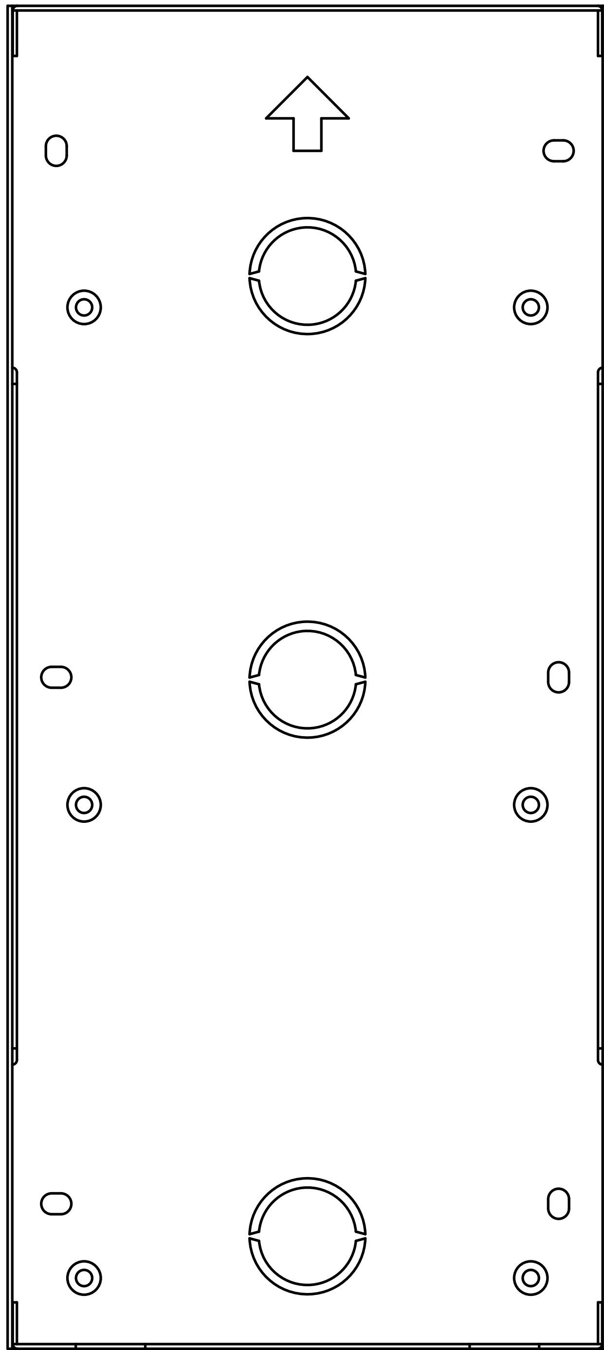
2 FRONT VIEW:FLUSHING MOUNTING BOX PLACEMENT
