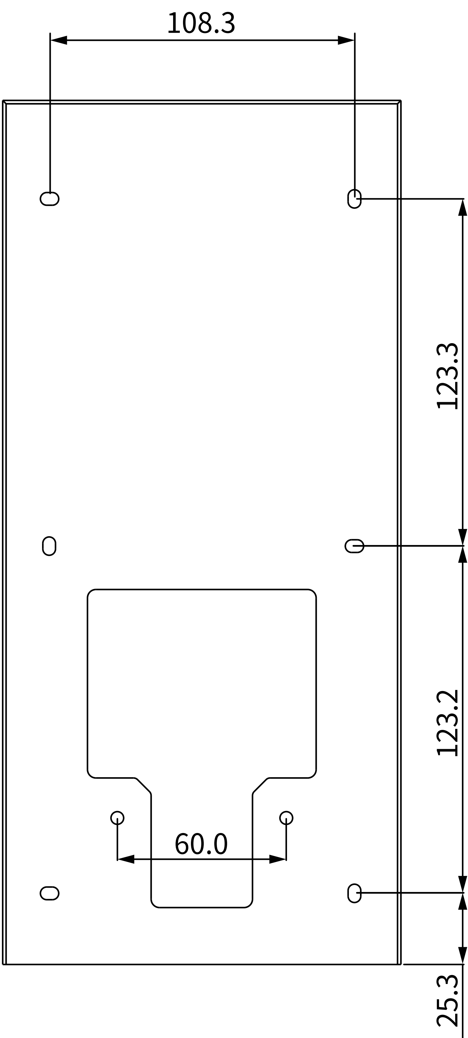
4 BACK VIEW
