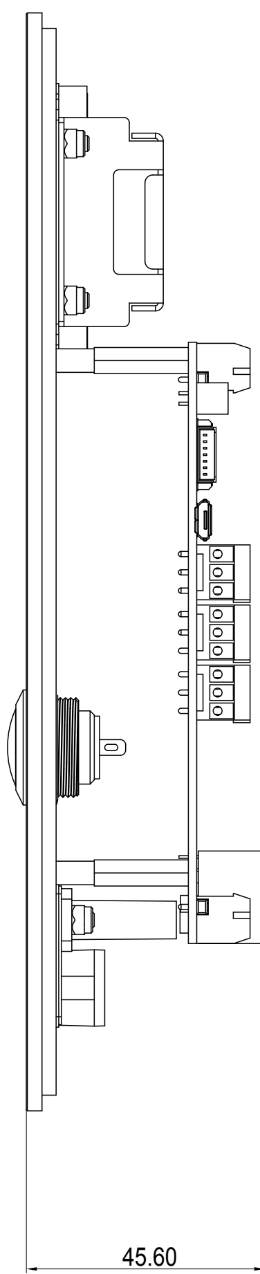
3 LEFT VIEW
