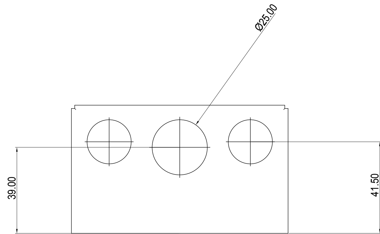
5 TOP VIEW
