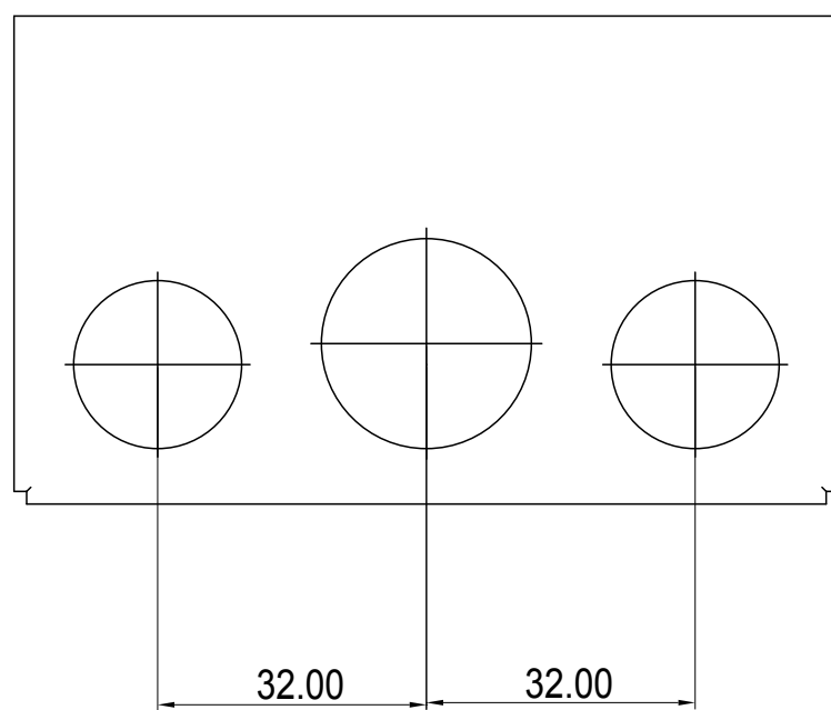
6 BOTTOM VIEW
