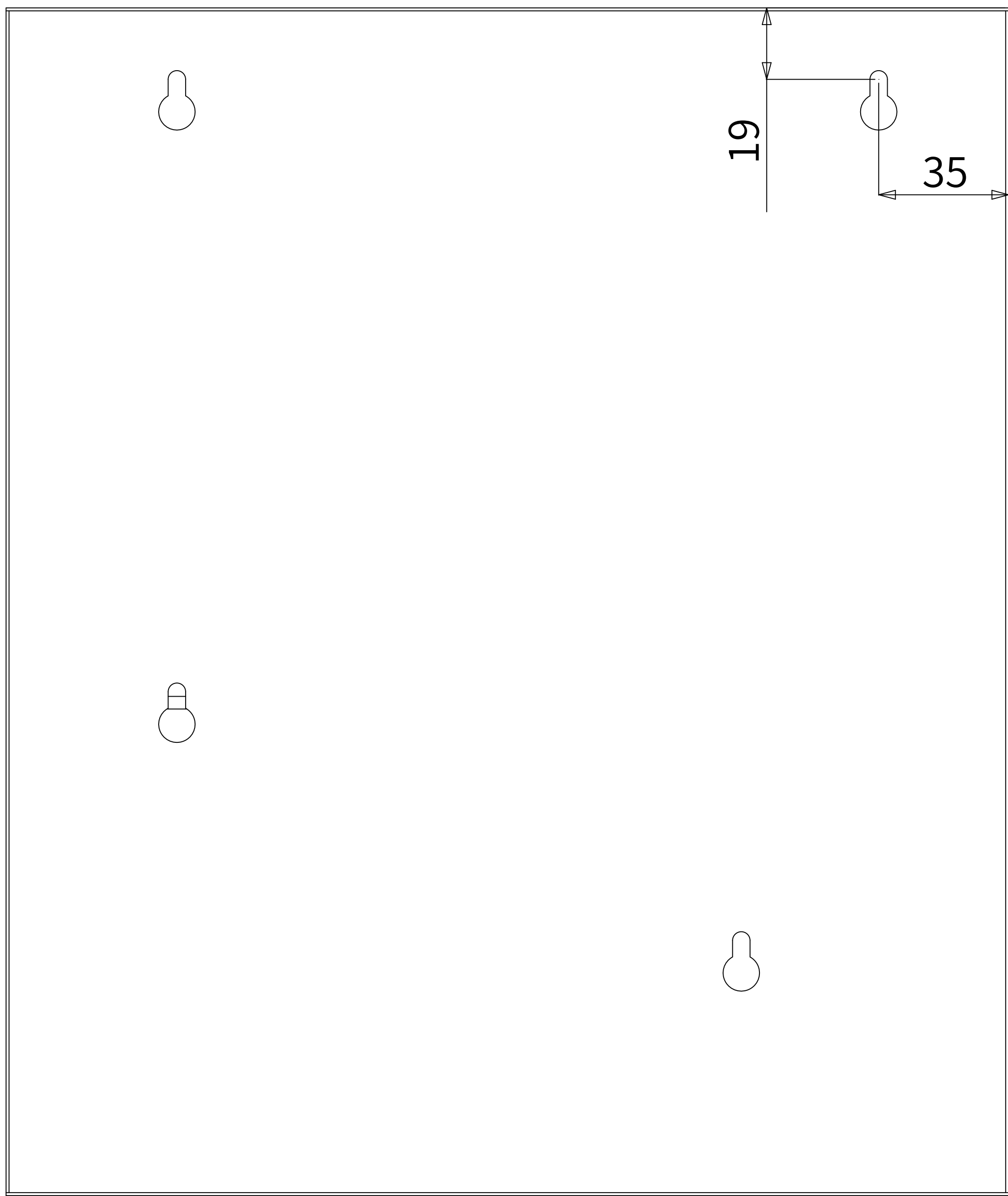
4 BACK VIEW
