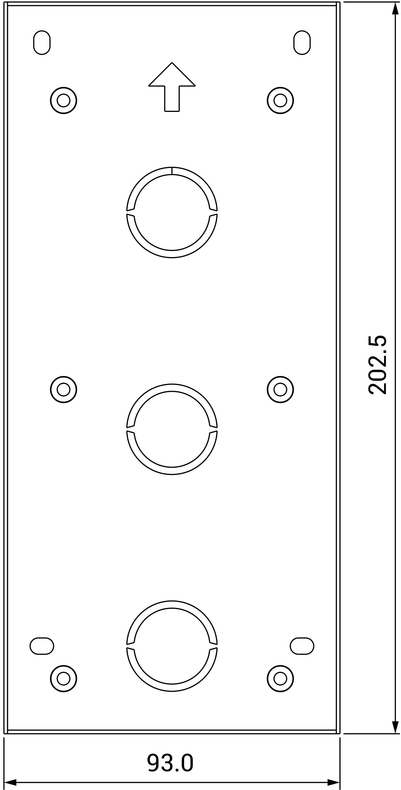
1 FRONT VIEW
