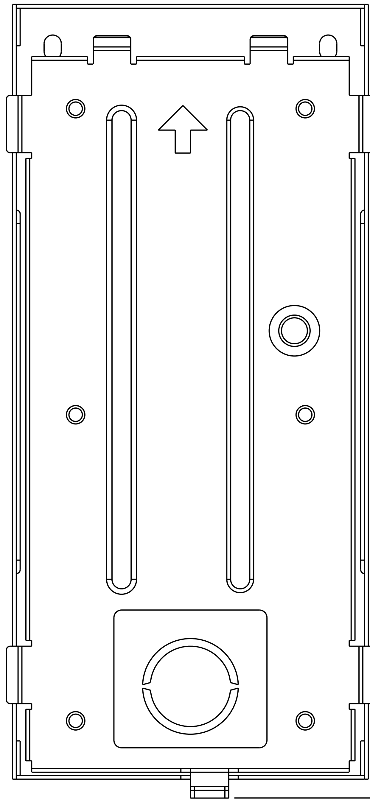
② FRONT VIEW:FLUSHING MOUNTING BOX PLACEMENT
