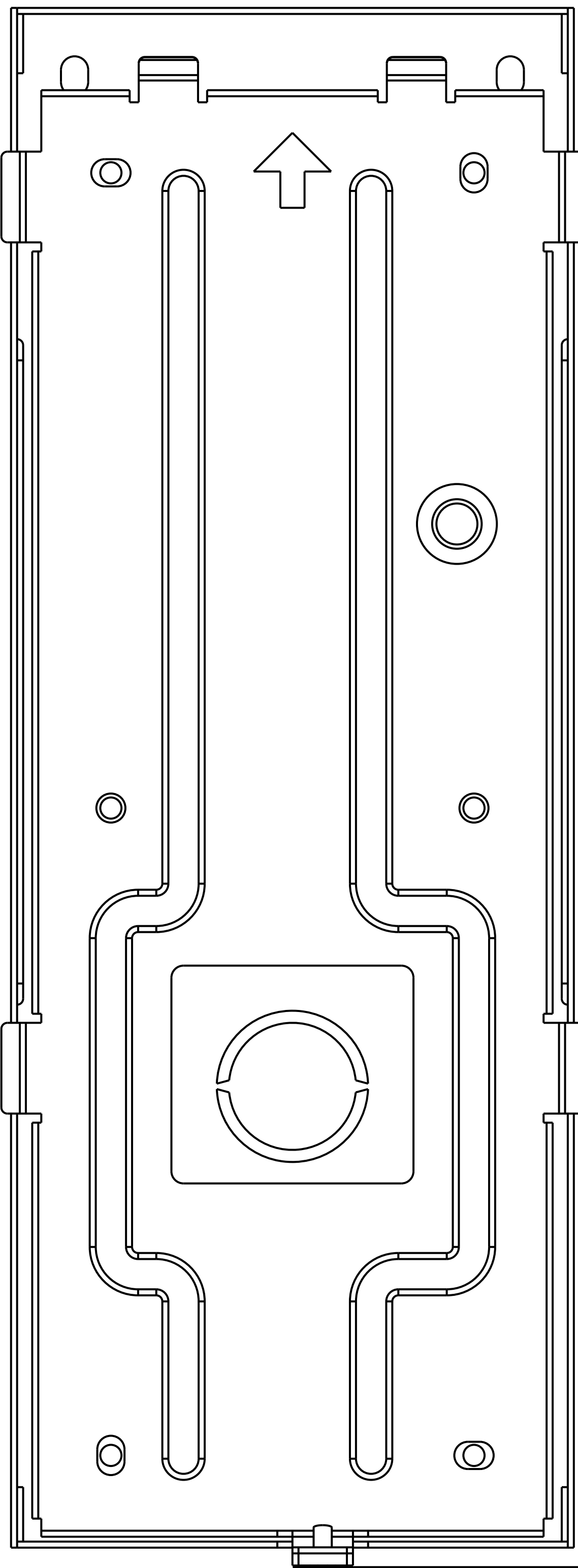
② FRONT VIEW:FLUSHING MOUNTING BOX WITH MODULE PLACEMENT
