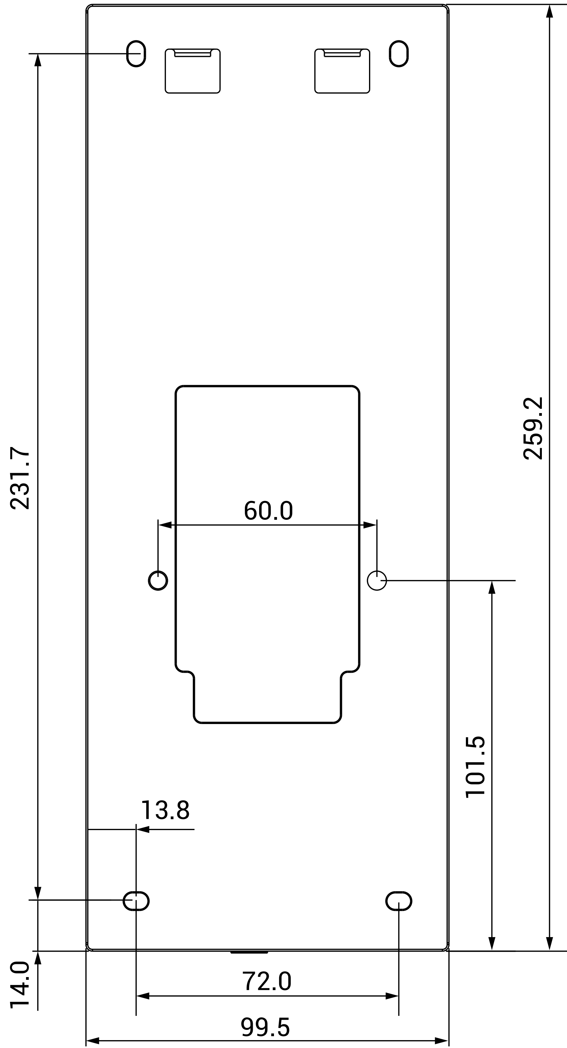
1 FRONT VIEW
