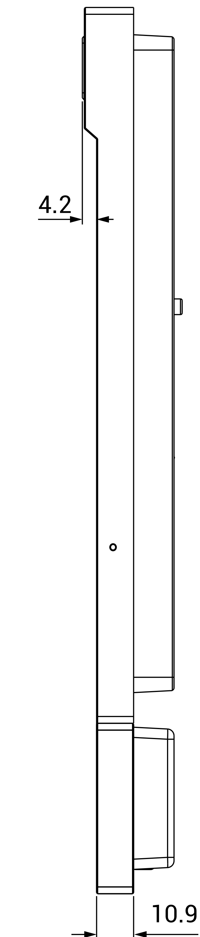
② RIGHT VIEW
