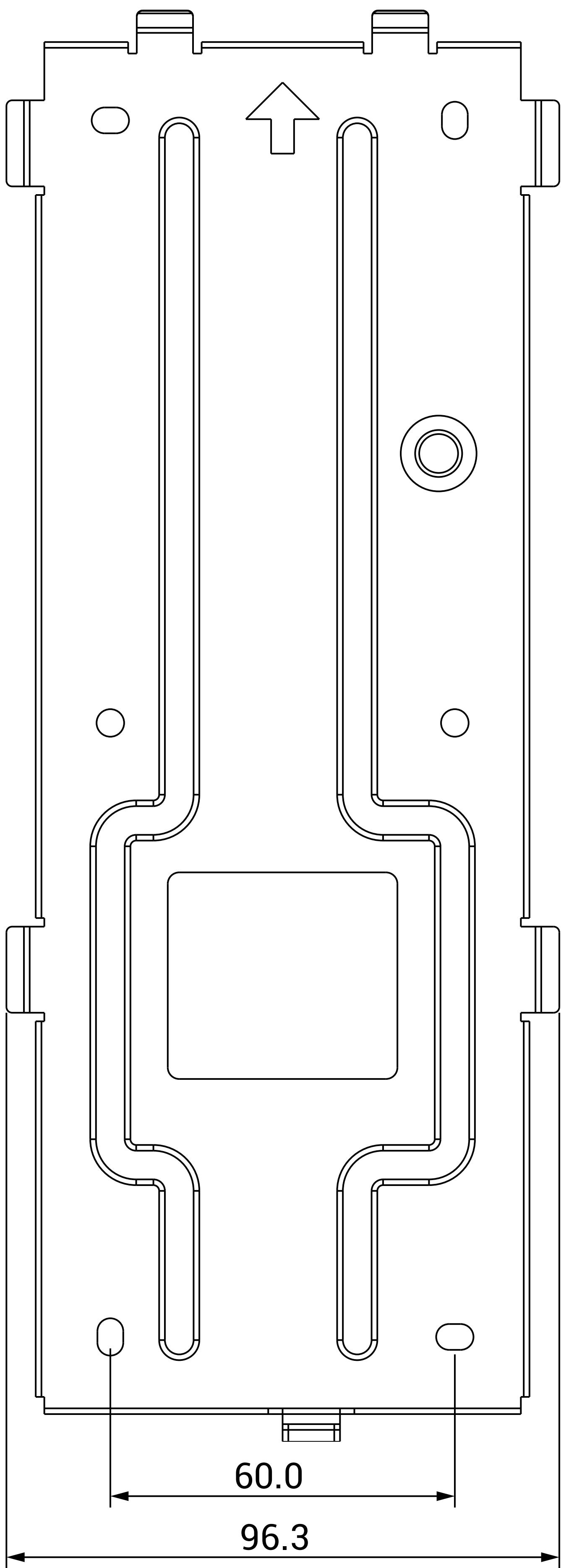
1 FRONT VIEW
