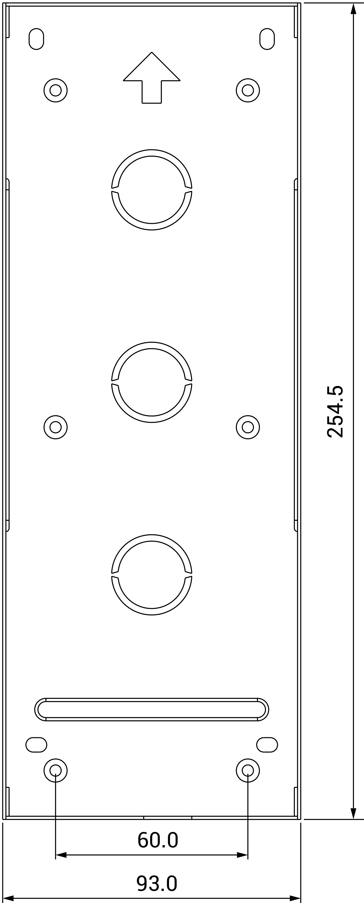
1 FRONT VIEW
