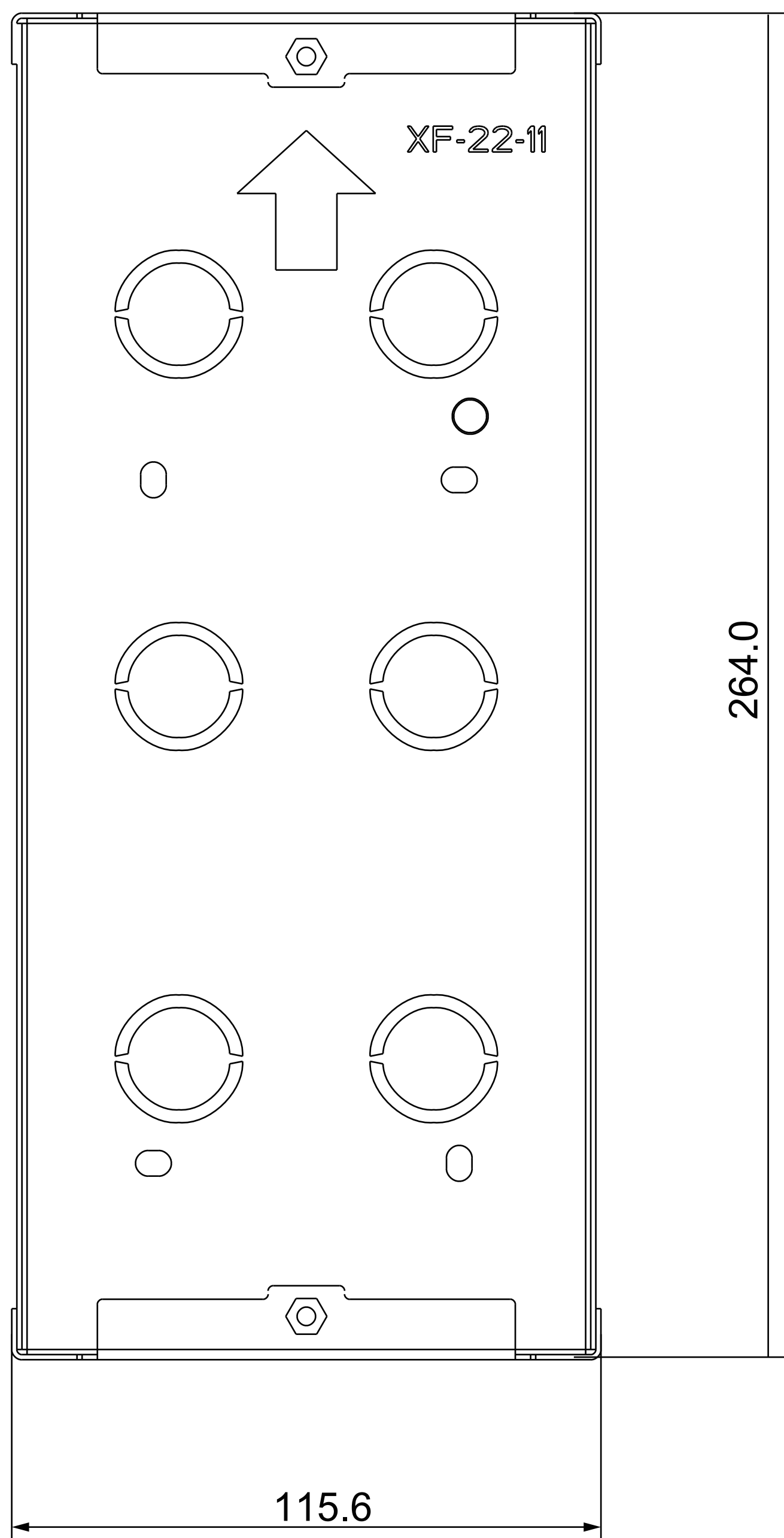
1 FRONT VIEW
