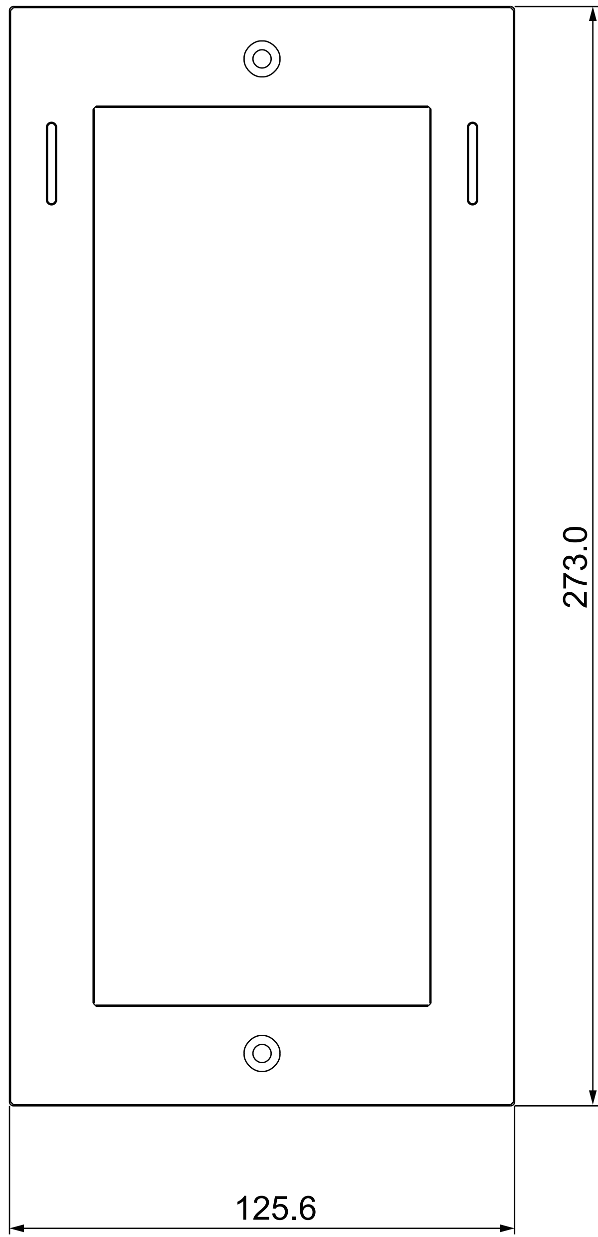
1 FRONT VIEW
