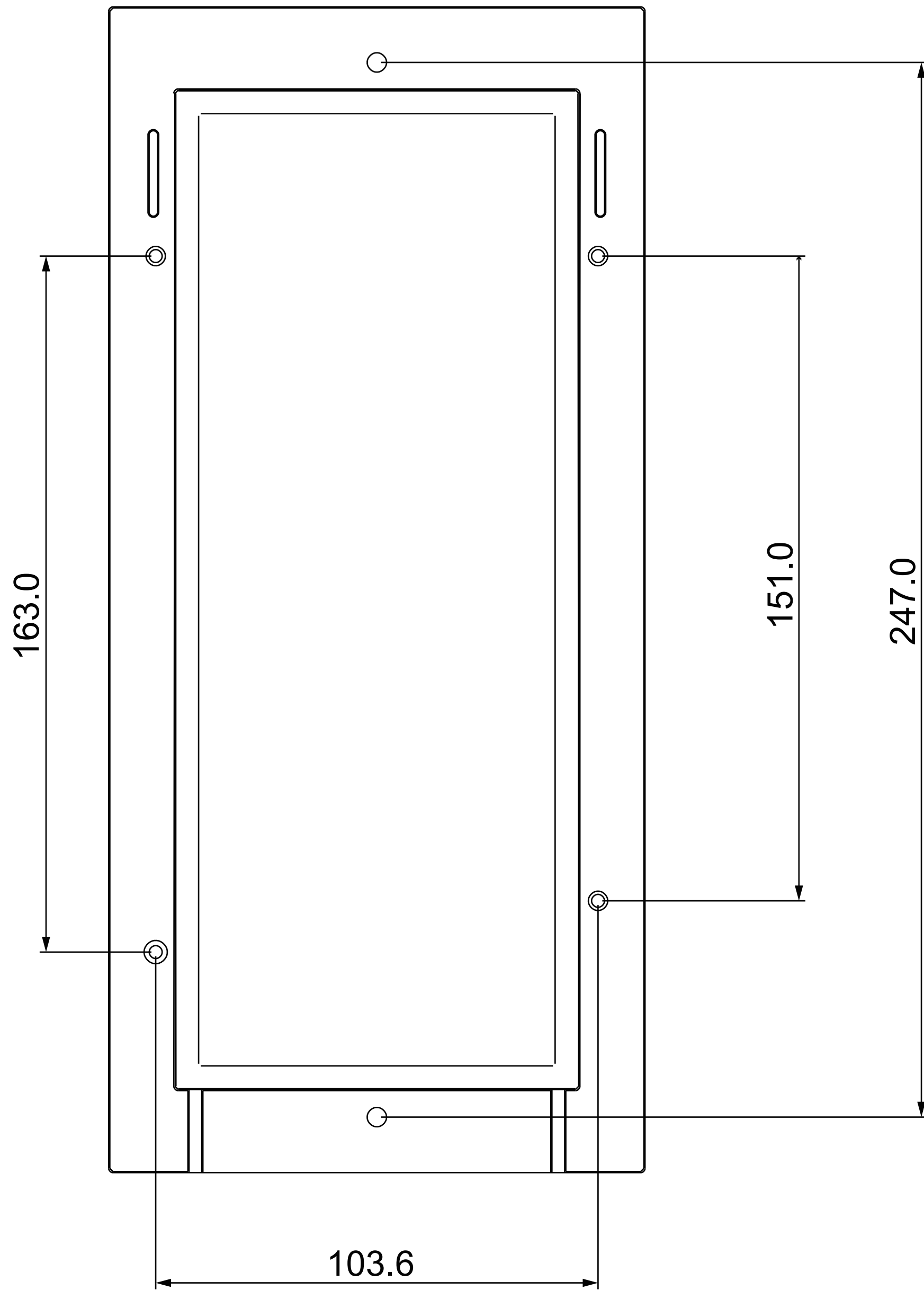
4 BACK VIEW
