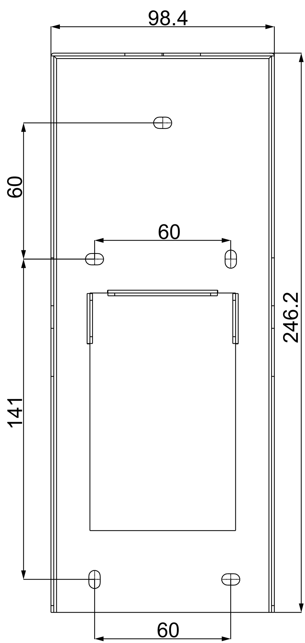
1 FRONT VIEW
