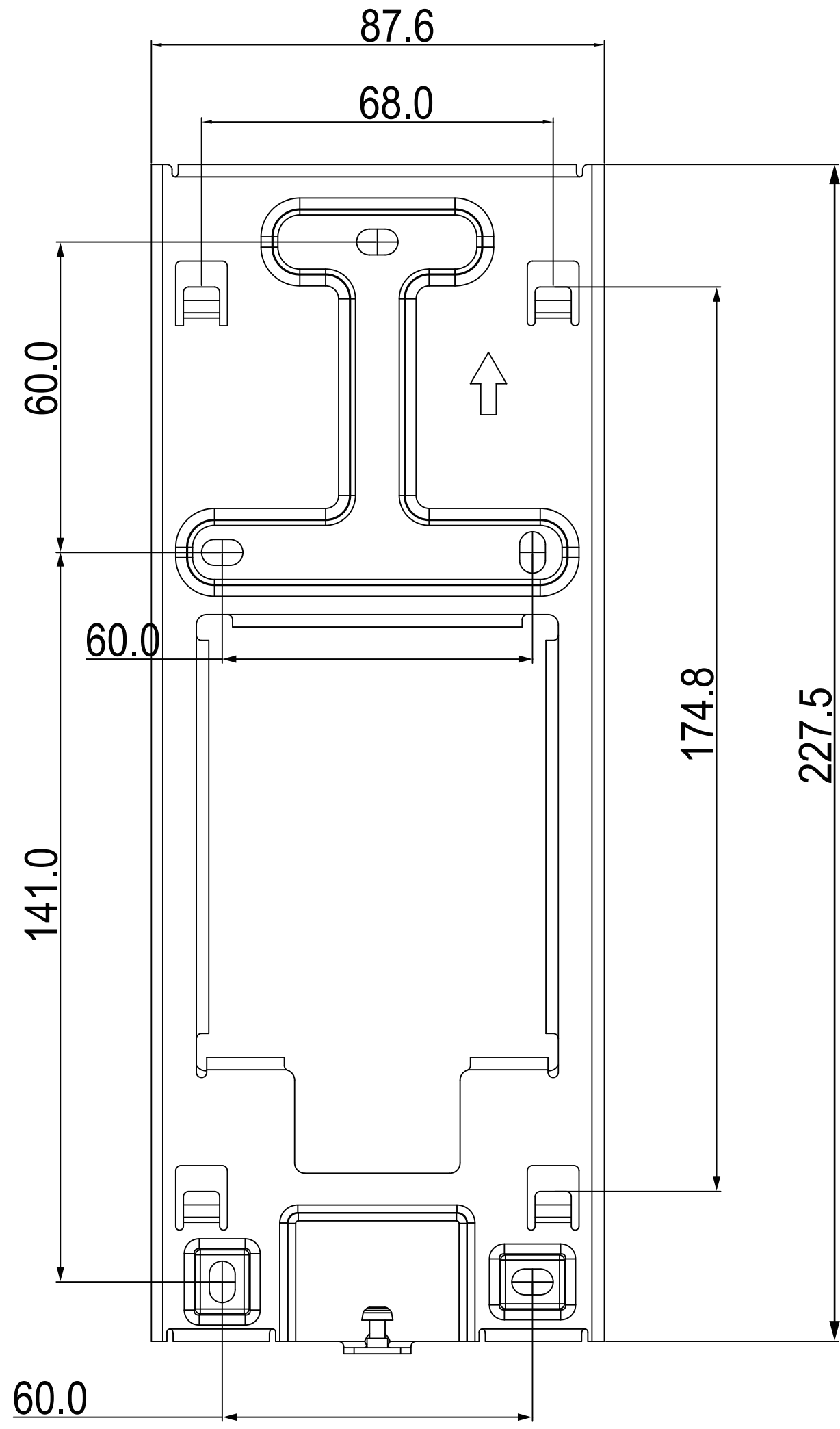
1 FRONT VIEW
