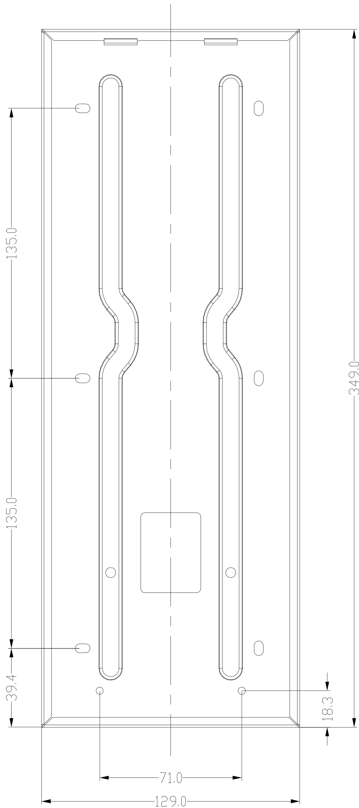
1 FRONT VIEW
