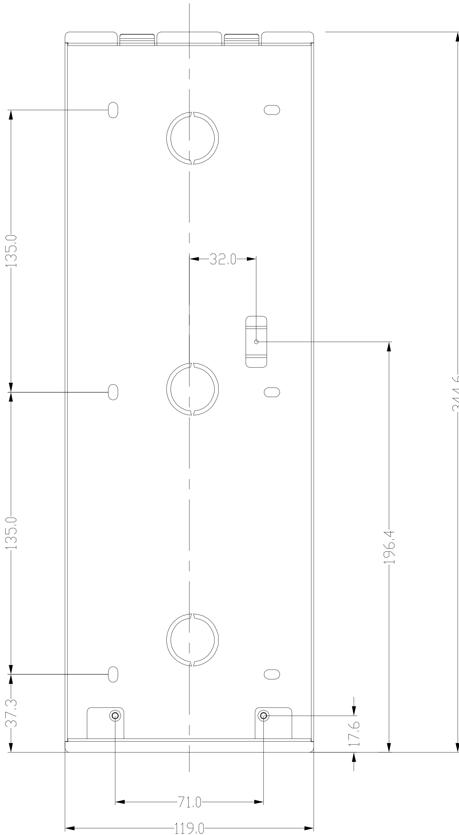
1 FRONT VIEW
