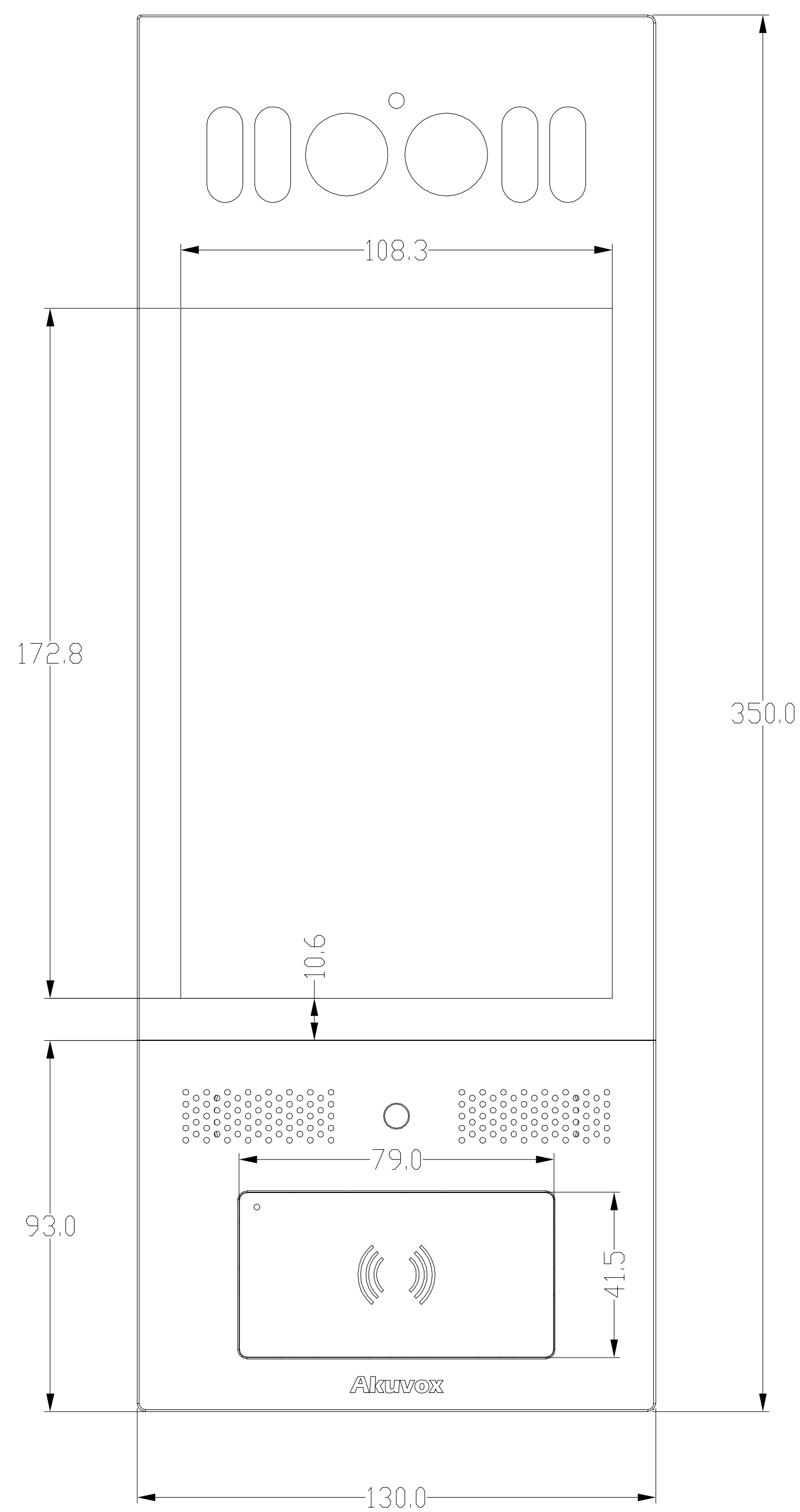
1 FRONT VIEW
