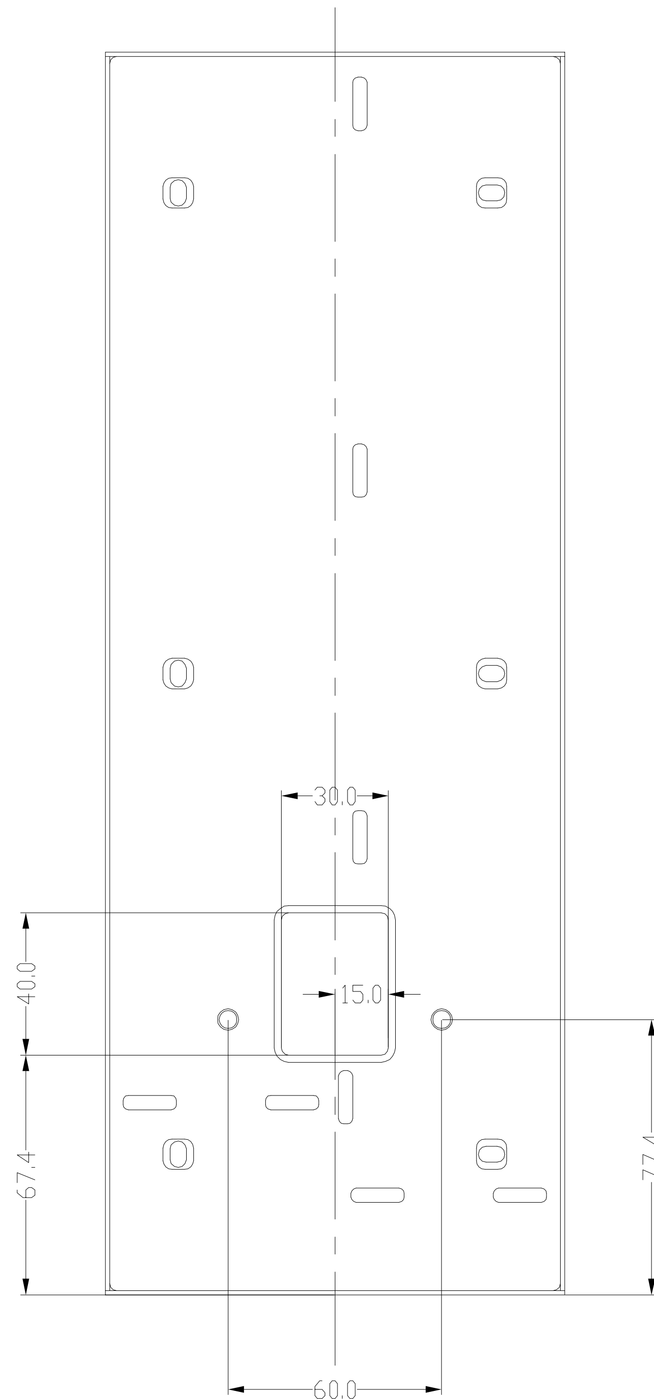
4 BACK VIEW
