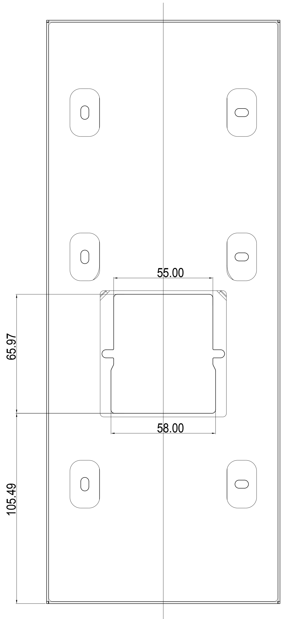
4 BACK VIEW
