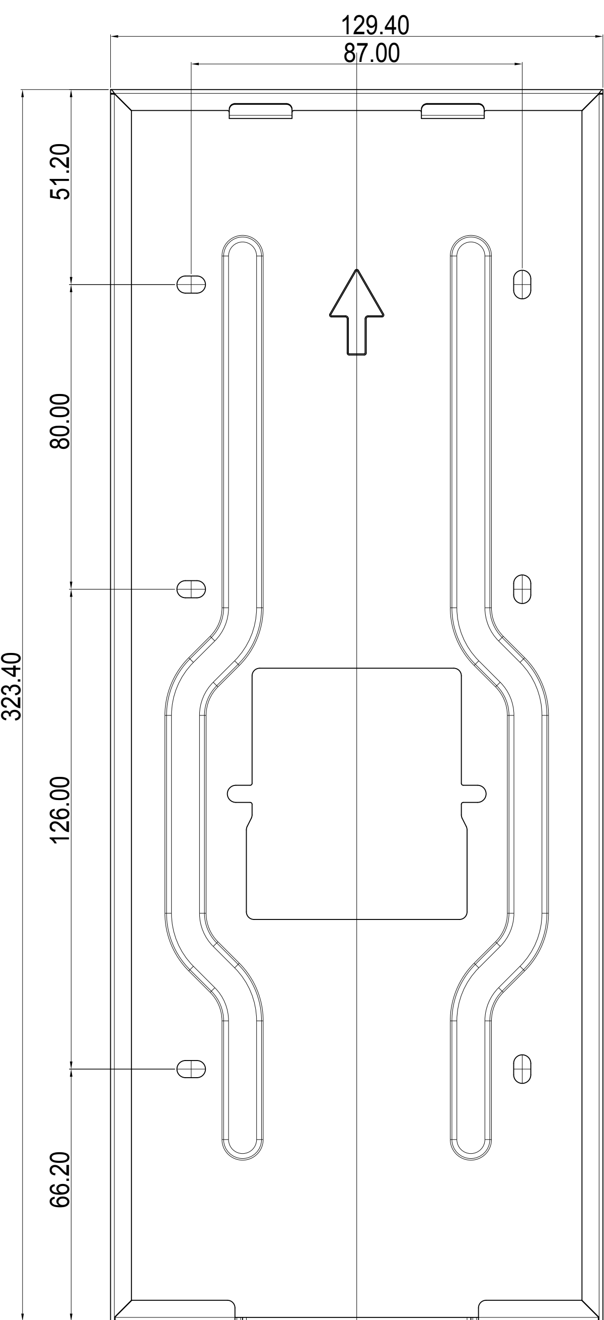
1 FRONT VIEW
