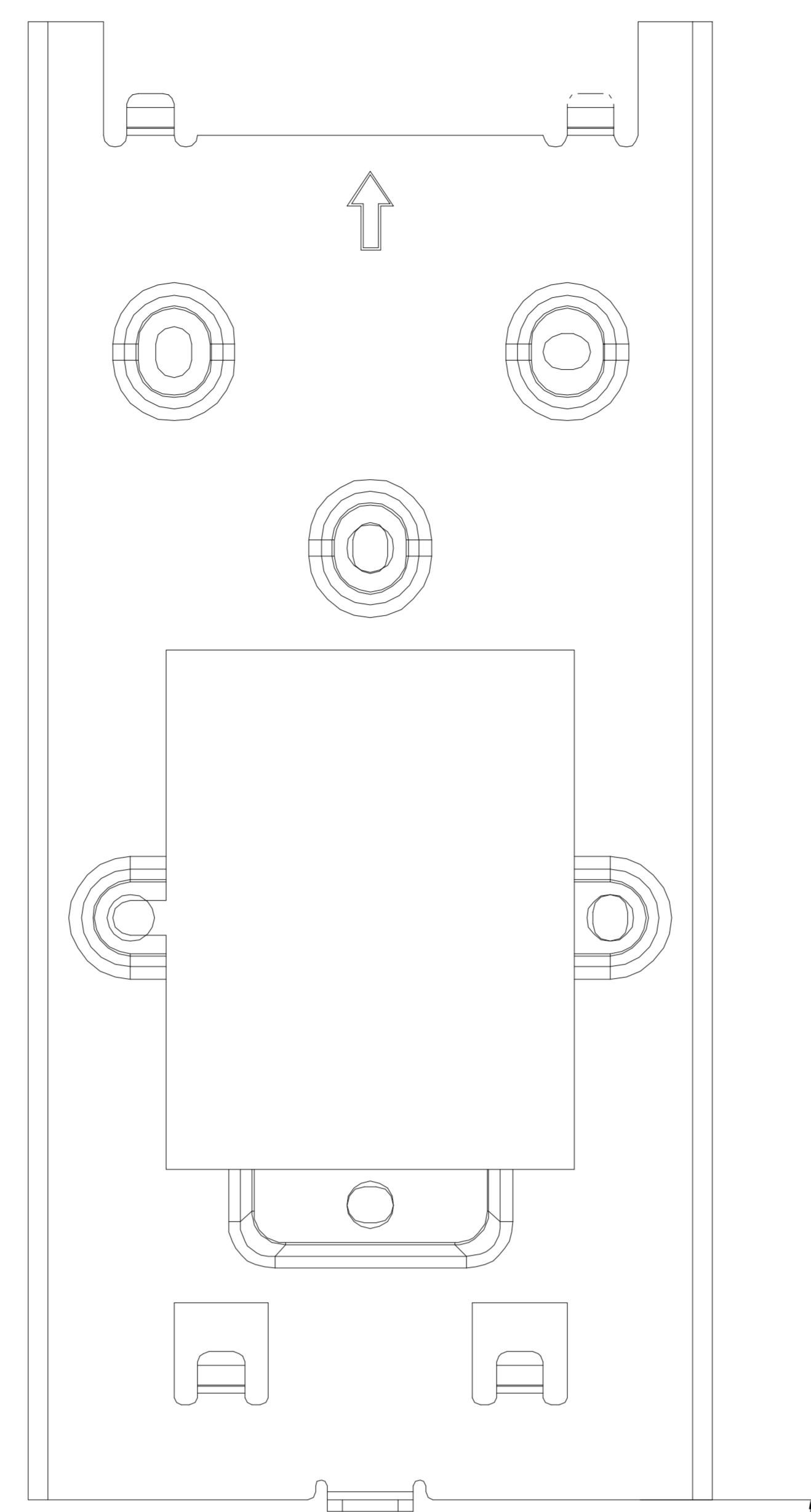
2 FRONT VIEW:WALL MOUNTING BRACKET PLACEMENT
