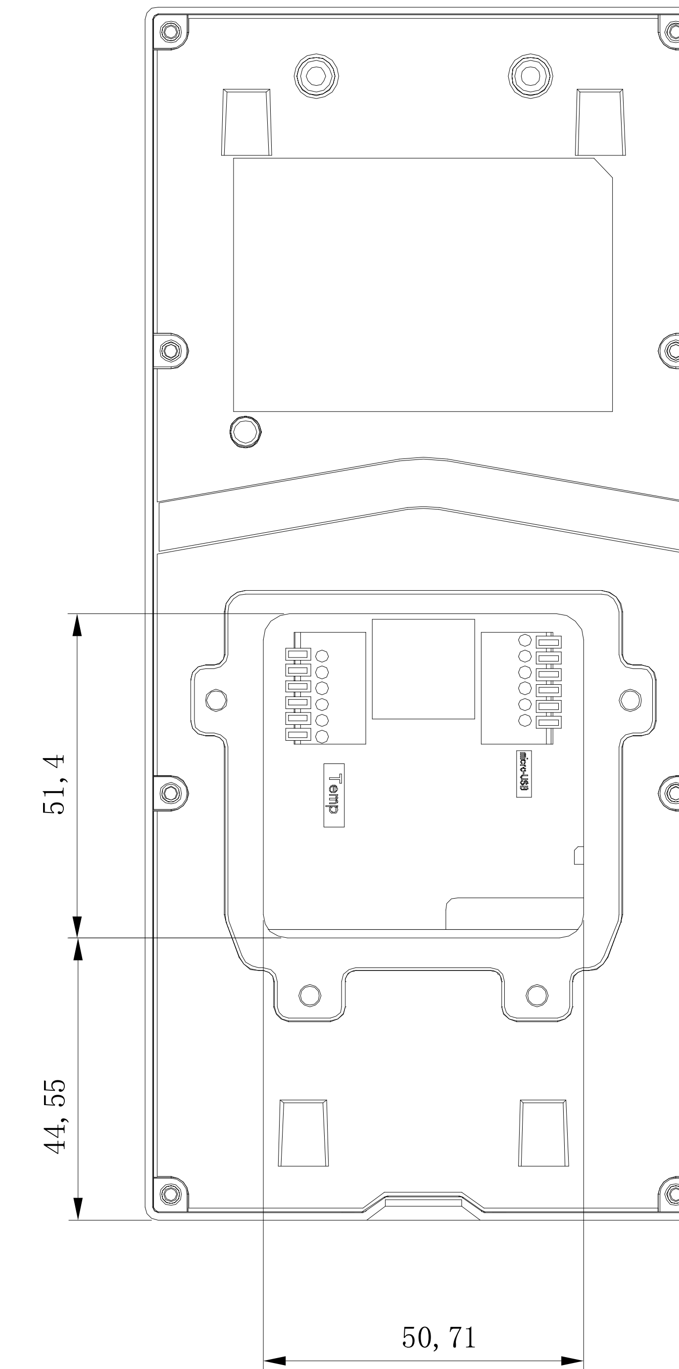
4 BACK VIEW
