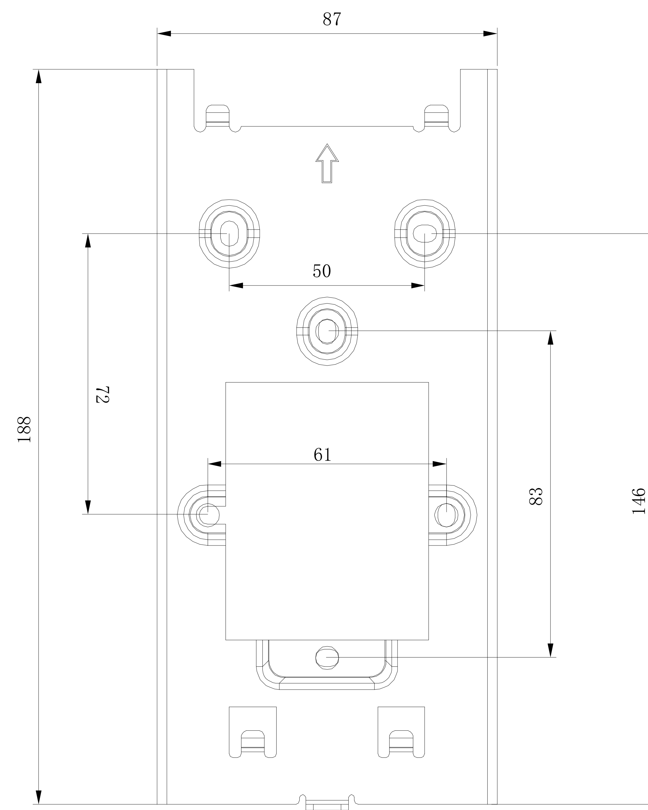
1 FRONT VIEW
